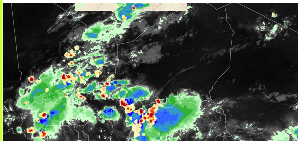
Figure 3: Image SAT du 29/09/2026 à 19h20 UTC (source: EUMETSAT)
